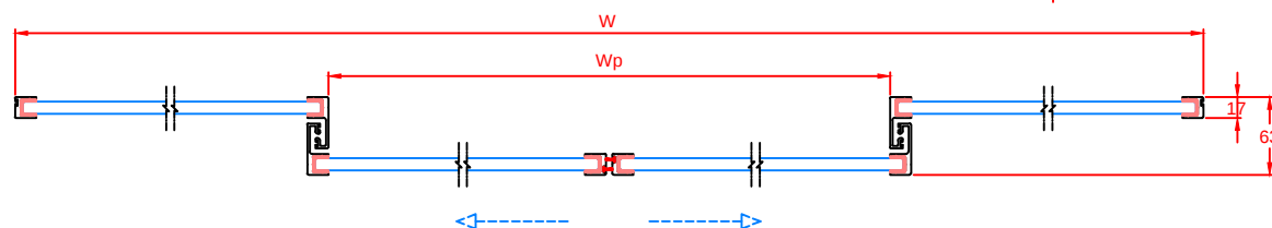
Section B-B
