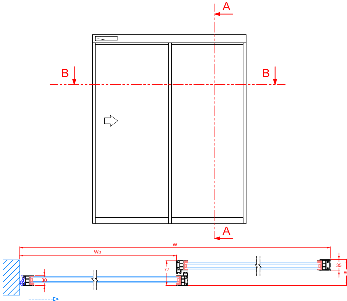
Section B-B
