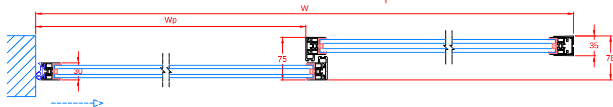
Section B-B
