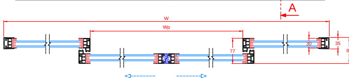
Section B-B
