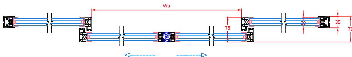
Section B-B
