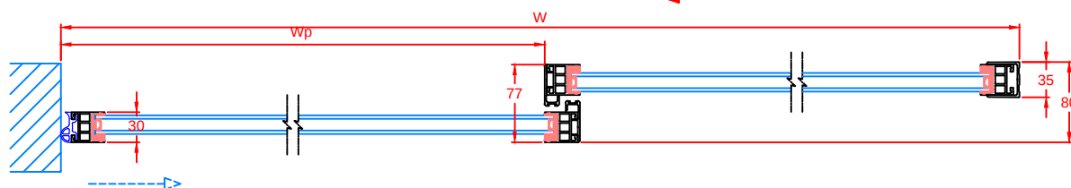
Section B-B
